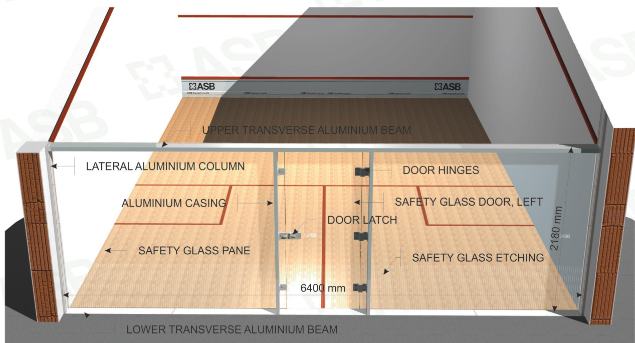
Front axonometric view
